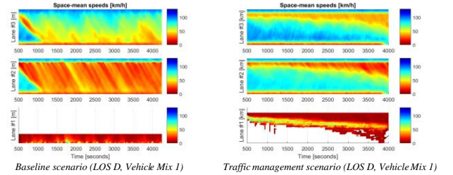
Figure 5. Comparison of the aggregated time-space diagrams per lane for use case 1.3 simulation experiments for LOS D and vehicle mix 1 (each time, top: left lane, middle: right lane, bottom: emergency lane/off-ramp), in the baseline (left column) and traffic management (right column) scenarios.
