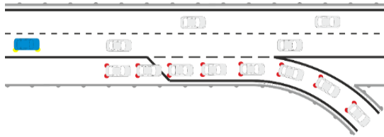
Figure 4. Detail view of the merging area in SUMO for scenario 1. The grey lane is the emergency lane, but opened temporarily to provide a possibility to house the upstream flowing queue. Colours indicate the vehicle type (yellow for legacy vehicles, blue for CAVs, and white for CVs).
